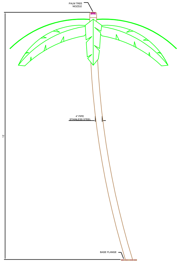
ELEVATION VIEW
