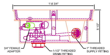
ELEVATION VIEW
