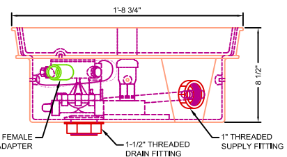
ELEVATION VIEW
