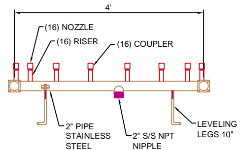
ELEVATION VIEW
